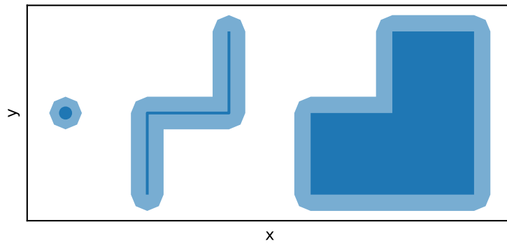
s.buffer(0.2, quad_segs=2)
