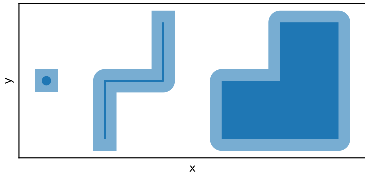
s.buffer(0.2, cap_style="square")
