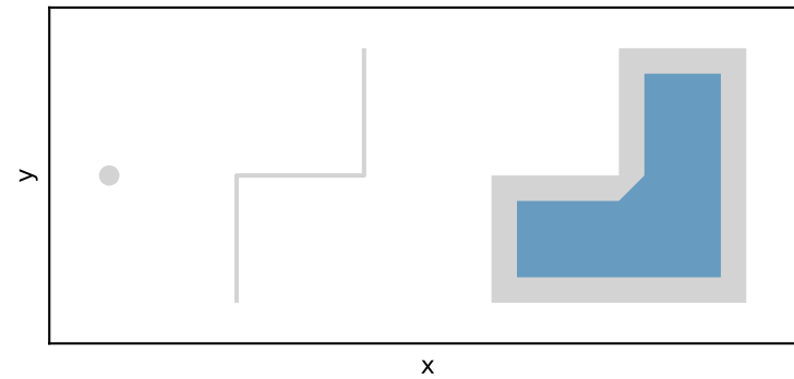
s.buffer(-0.2, join_style="bevel")
