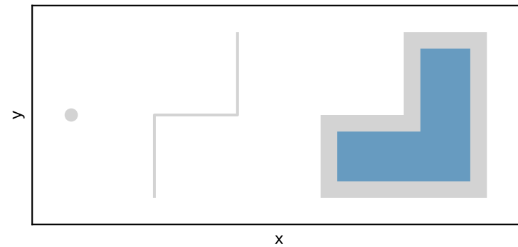
s.buffer(-0.2, join_style="mitre")
