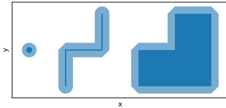
s.buffer(0.2, join_style="bevel")
