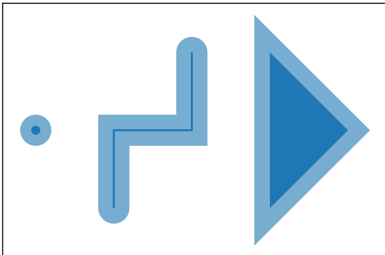
s.buffer(0.2, join_style="mitre")
