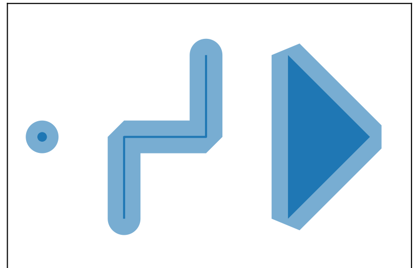
s.buffer(0.2, join_style="bevel")
