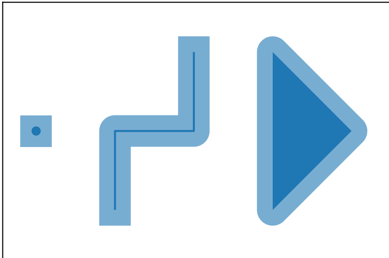
s.buffer(0.2, cap_style="square")
