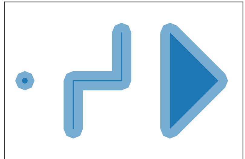
s.buffer(0.2, resolution=2)
